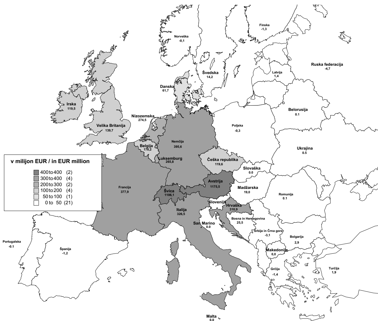
Figure 2: DI value of European countries in Slovenia at the end of 2003
